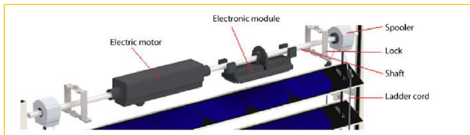
Figure 5.2. Arrangement of elements under the casing
