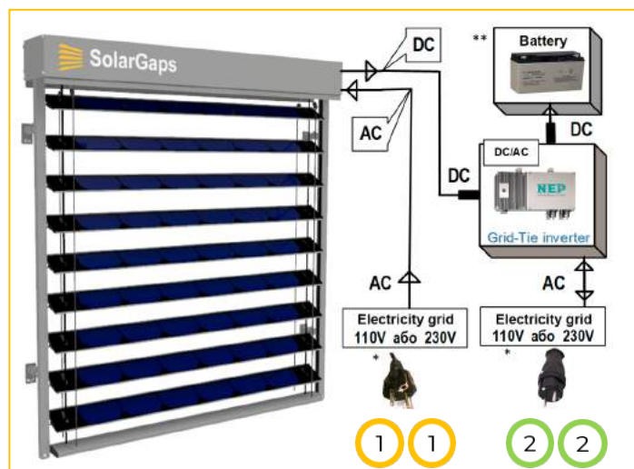
Diagram for connection of the product
